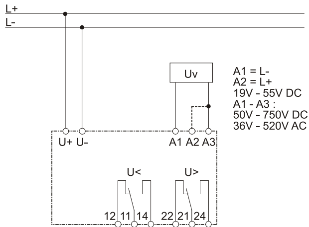
Figure 2.1: Connection XU1-DC-1
