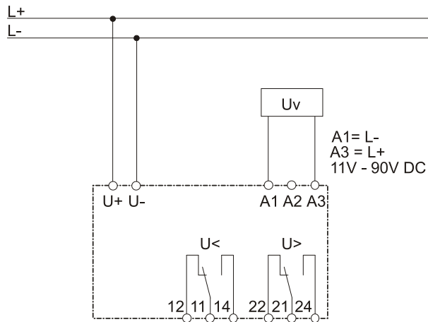
Figure 2.2: Connection XU1-DC-2
