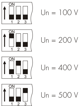
Figure 4.4: Adjustment of rated voltage XU1-DC-1
