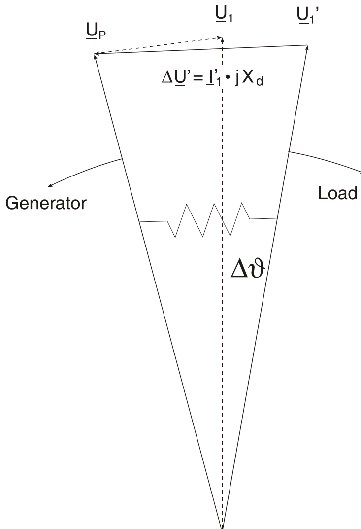
Figure 3.4: Voltage vectors at mains failure
