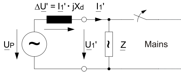
Figure 3.3: Equivalent circuit at mains failure
